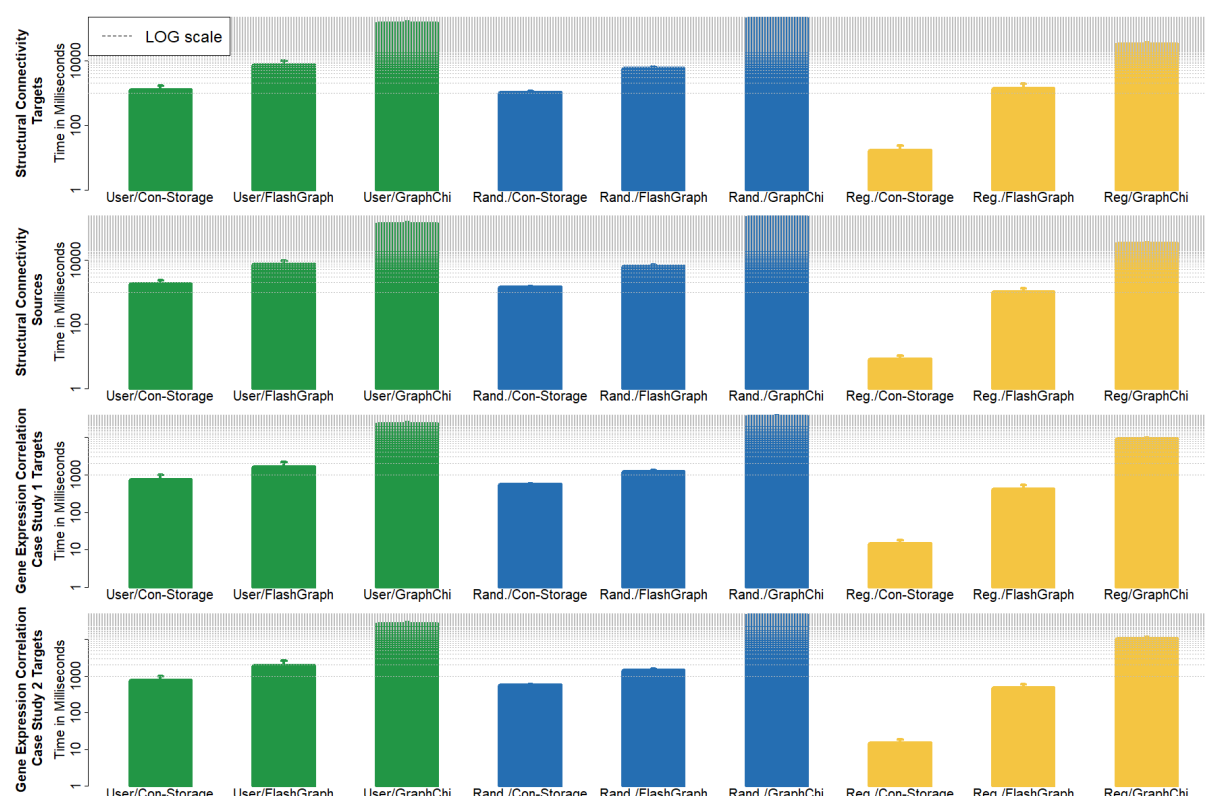
Figure 10: Comparison of query speed with state-of-the-art tools. Bars show the mean query-time with standard error of 10 user-defined VOI queries (green), 100 random VOI queries (blue) and 10 region VOI queries (yellow), for the Connectivity Storage, FlashGraph and GraphChi. The bars are log scaled, indicated by equidistant grey dotted lines (distance between two lines represent 1 second).
