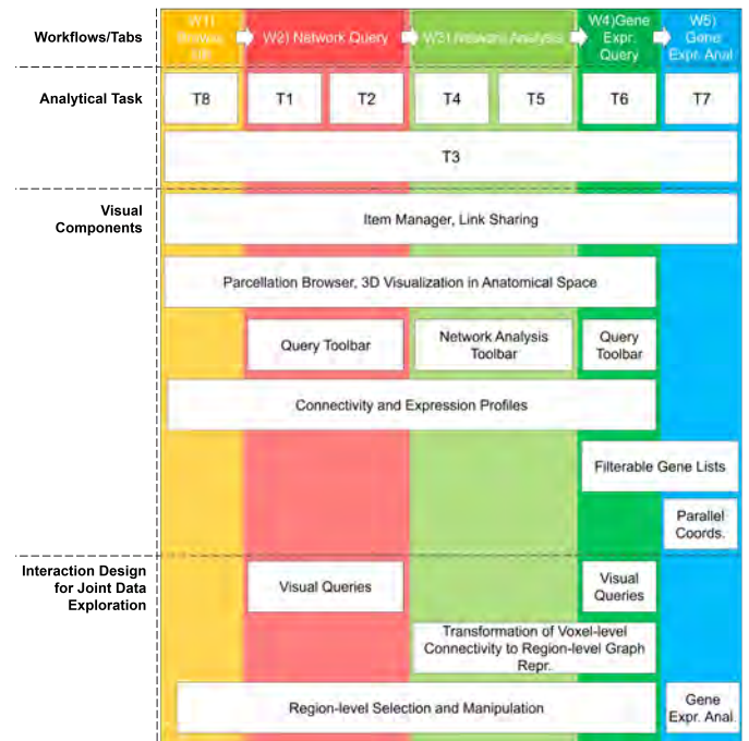
Fig. 4. Association of the workflows/tabs (Section 5), analytical tasks (Section 3.3), visual components (Section 6), and interactions for joint data exploration (Section 7). The components and interactions are arranged by their order of appearance in the main text.
