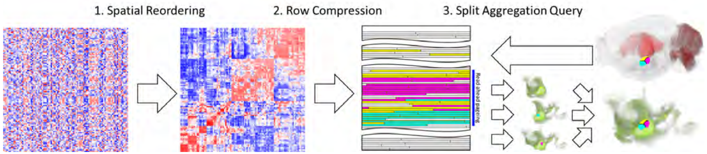
Fig. 2. Principle of the Connectivity Storage and real time Aggregation Queries: 1. Spatial reordering of a (voxel-level) connectivity matrix. Rows/columns that represent the outgoing/incoming connectivity of voxels are reordered, so that rows/columns that belong to spatially close voxel are close to each other. 2. Row Compression: The reordered connectivity matrix is stored with a row-wise compression as Connectivity Storage File on the hard disk. This saves disk space (and therefore reading time) by exploiting sparseness. 3. Split Aggregation Query: A VOI (yellow, purple and cyan indicates anatomical sub-regions of the VOI) is selected on 3D spatial data (e.g. spatial gene expression data, red). Outgoing connectivity is aggregated by reading the corresponding rows (yellow, red and cyan) from the Connectivity Storage File into three separate Connectivity Volumes . Since spatially close rows are also close in the file, they can profit from read-ahead paging (blue). Aggregated of the VOI can be generated from the three individual Connectivity Volumes (green) but is also available for the 3 subregions (e.g. for region-level graph representation).
