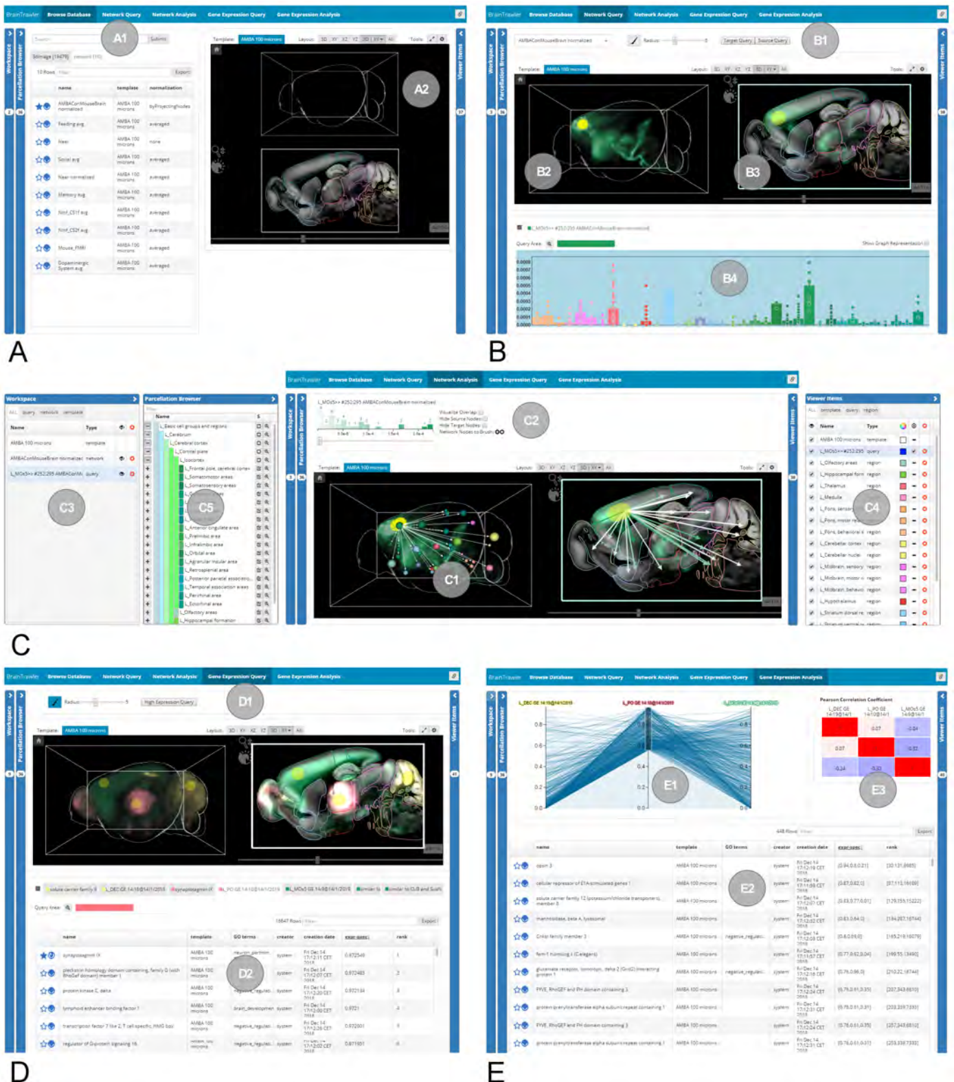
Fig. 1. Task-based web-component for iterative exploration of multiscale brain data. Detailed views of the individual tabs/subfigures can be seen in the supplement. A) Browse Database tab: The user can browse a collection of 3D gene expression and connectivity data via a text search (A1) and visualize the data directly in the 3D view (A2) or add it to the workspace (C3). B) Network Query tab: The user can execute target/source queries from the Query Toolbar (B1) on connectivity matrices that have been added to the workspace. Gene expression/Connectivity is rendered volumetrically in a 3D view (B2), in a 2D slice view (B3) and as region-wise quantitative representation (Expression/Connectivity Profile) (B4). C) Network Analysis tab: The user can explore networks or connectivities on a region level in a ball/stick representation (C1), controlled by the Network Analysis Toolbar showing histograms of the visualized graphs and threshold sliders for edge filtering (C2). The workspace manages which items (3D volumetric data, networks, query results) are shown in each tab (C3) while the Viewer Items List (C4) controls their appearance (e.g. color). The Parcellation Browser (C5) shows a hierarchical (anatomical) brain parcellation and is used to change the parcellation level of visualized graphs and profiles. D) Gene Expression Query tab: Via the Query Toolbar (D1), Gene Expression Queries can be executed. Resulting gene lists are shown in a table below (D2). E) Gene Expression Analysis tab: Gene lists can be compared in a parallel coordinate system (E1). Its selection is shown in a table (E2), its correlation in a heatmap (E3).
